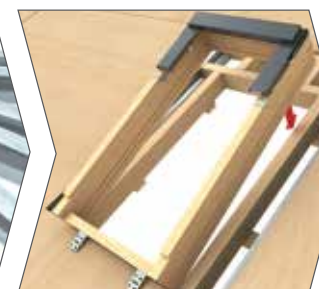
Install roof window frame
